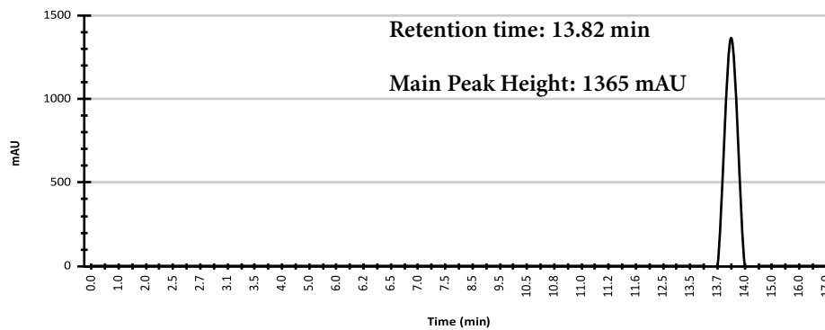
HPLC Chromatogram
